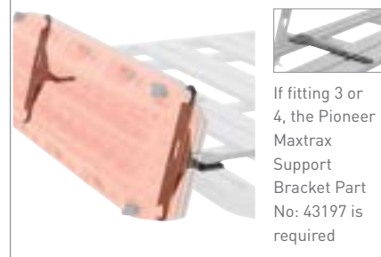
12.16 RECOVERY TRACK SIDE ANGLE BRACKET
